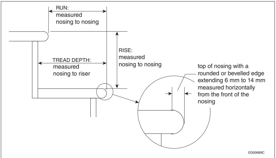
FIGURE 14 - Stair Detail
