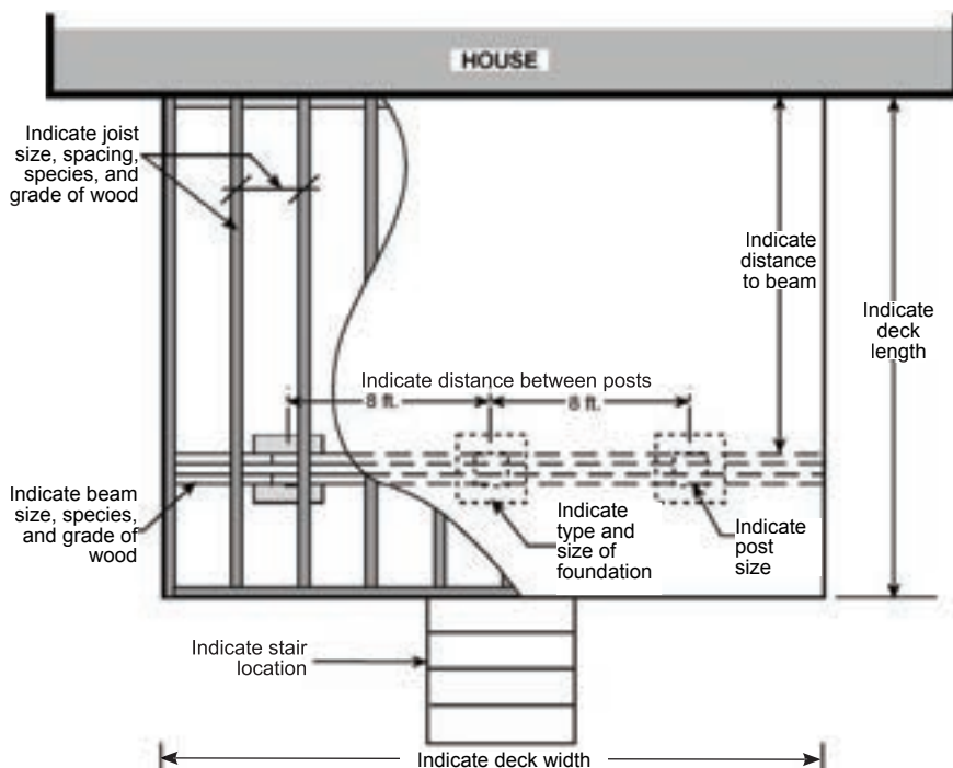
FIGURE 2 - Typical Construction Plan
