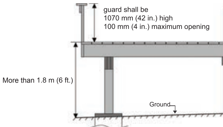
FIGURE 12 - Guardrail Height
