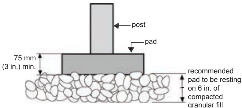
FIGURE 5 - Surface Pad Foundation
