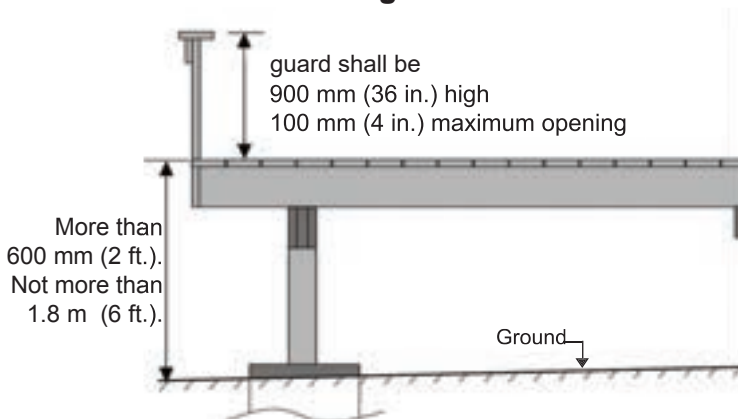
FIGURE 11 - Guardrail Height
