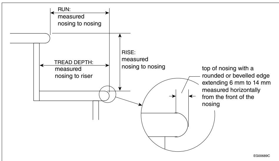
FIGURE 14 - Stair Detail
