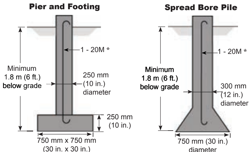
FIGURE 6 - Piles or piers
