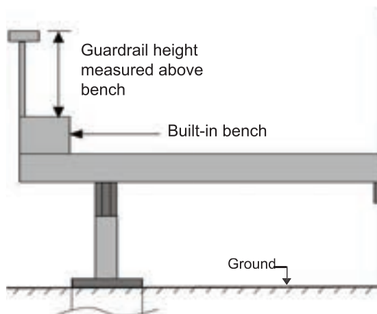
FIGURE 13 - Guardrail and Bench
